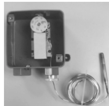
Fig. 1 -- Interior of an A19ANC thermostat.
